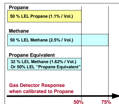
Figure 4 Propane Equivalent response
