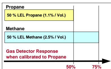
Figure 3 Propane and methane response on a propane calibrated detector
