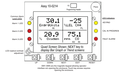
Figure 1-2. Front Panel Display (open enclosure)
