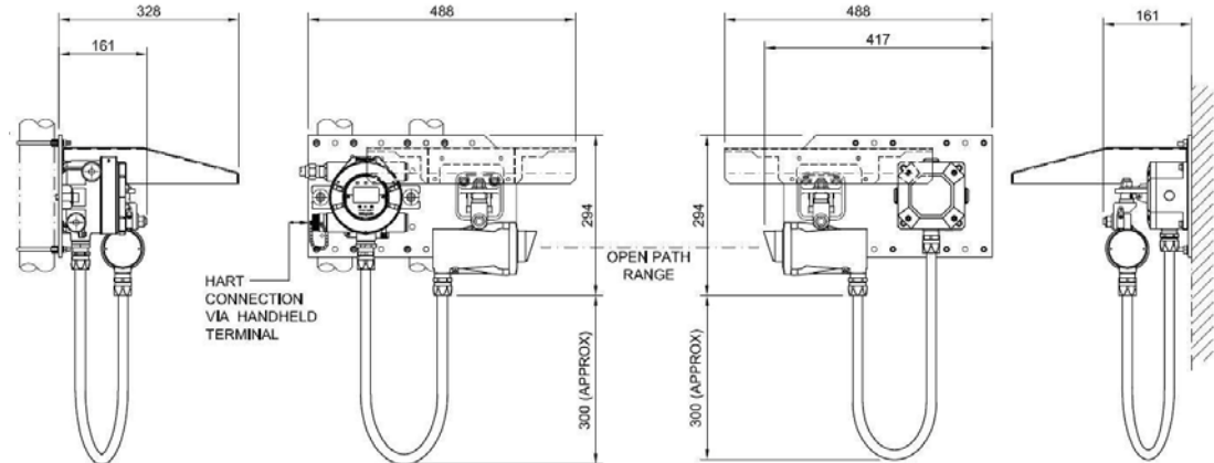
EXCEL RECEIVER ASSEMBLY (INC. DETAILS FOR 2" N.B PIPE MOUNT APPLICATIONS)
