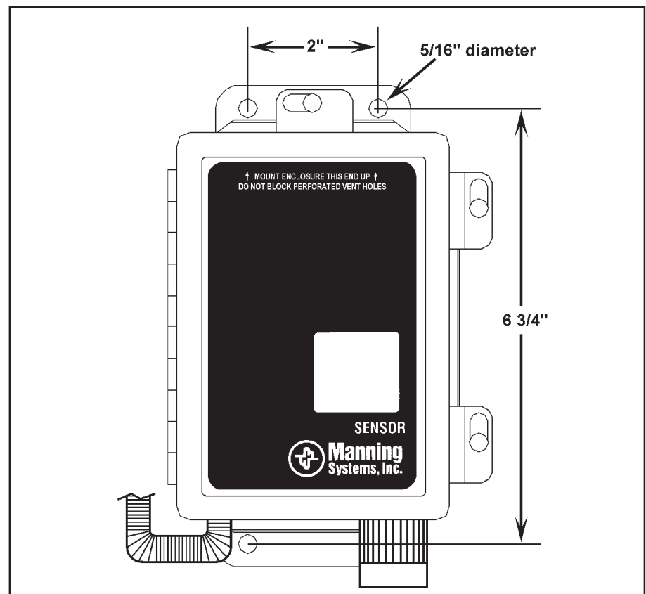
Figure 1: Mounting dimensions for the EC-F2 Sensor
